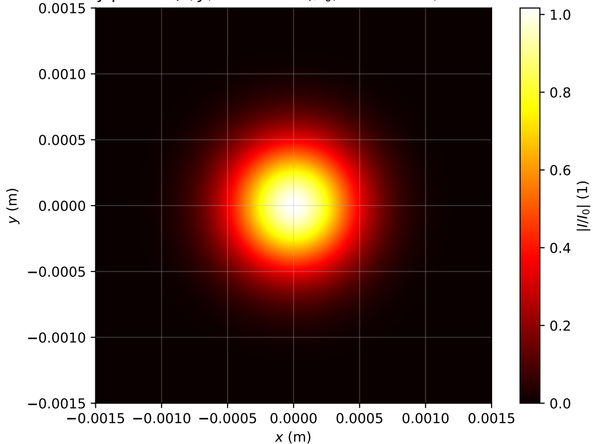
Intensity profile I(x, y, z = 0.398m)/I_0 , P_{in}=0.4P_{cr} , artificial time
